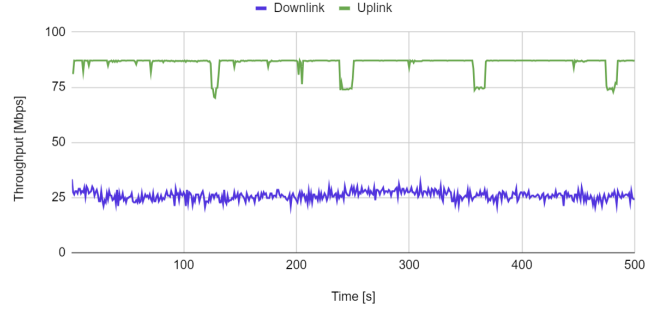
Fig. 5. Throughput of the CPE using L2 communication.
